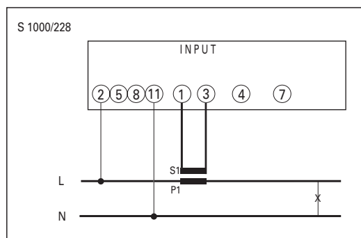
Single-phase network
