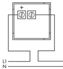
Direct connection
