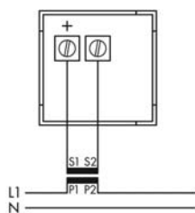
Connection to current transformer
